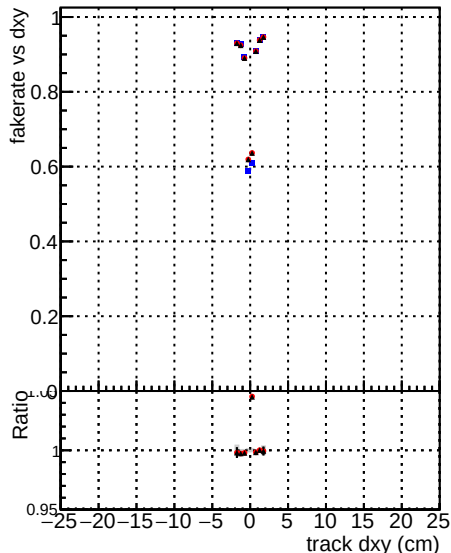
Fake rate vs d DOM V0001 R0000000001 Global cmssw RECO DOM V0001 R0000000001 Global mkFitOriginal RECO mkFitNewALL RECO
