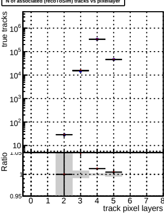
N of associated (recoToSim) tracks vs pixellayer
