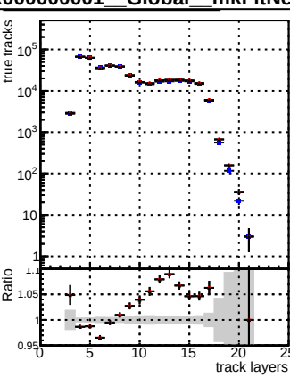
N of associated (recoToSim) tracks vs l
