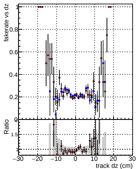
Global cmssw RECO Global mktreeOriginal RECO Global mktreeNewALL RECO DOM V0001 R0000000001 DOM V0001 R0000000001 DOM V0001 R0000000001 Global cmssw RECO Global mktreeOriginal RECO Global mktreeNewALL RECO DOM V0001 R0000000001 DOM V0001 R0000000001 DOM V0001 R0000000001
