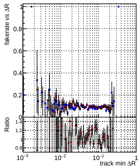
—●— DQM_V0001_R000000001_Global_cmssw_RECO —●— DQM_V0001_R000000001_Global_mkFitOriginal_RECO —●— DQM_V0001_R000000001_Global_mkFitNewALL_RECO
