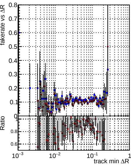
Legend: DQM_V0001_R000000001 Global cmssw RECO, DQM_V0001_R000000001 Global mkFitOriginal RECO, DQM_V0001_R000000001 Global mkFitNewALL RECO
