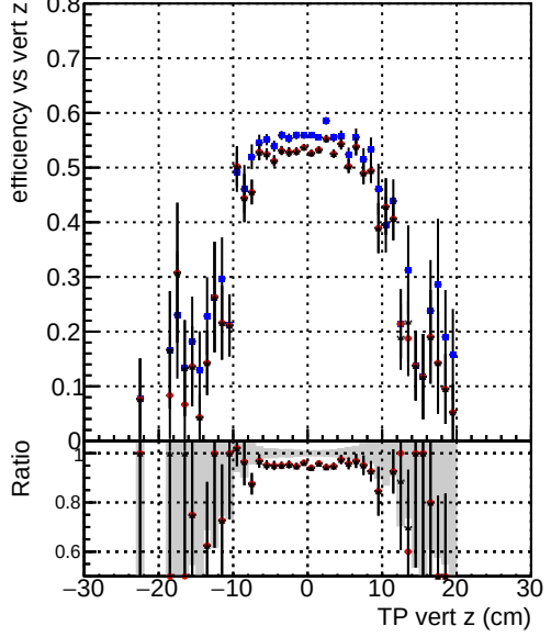
Efficiency vs. sim PV z —●— DQM_V0001_R000000001_Global_cmssw_RECO —●— DQM_V0001_R000000001_Global_mkFitOriginal_RECO —●— DQM_V0001_R000000001_Global_mkFitNewALL_RECO
