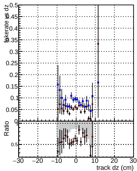
DOM_V0001 R0000000001 Global cmswv RECO Fake rate vs d Blue dots Red dots Black line Blue line Red line Duplicates Rate vs Dxy Blue dots Red dots Black line Blue line Red line Pileup rate vs dxy Blue dots Red dots Black line Blue line Red line
