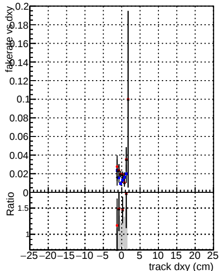
DOM V0001 R0000000001 Global cmswv RECO DOM V0001 R0000000001 Global mkFit Original RECO DOM V0001 R0000000001 Global mkFit NewALL RECO
