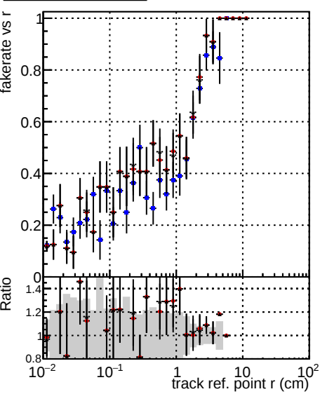
—●— DQM_V0001_R000000001 Global cmssw RECO —●— DQM_V0001_R000000001 Global mkFitOriginal RECO —●— DQM_V0001_R000000001 Global mkFitNewALL RECO
