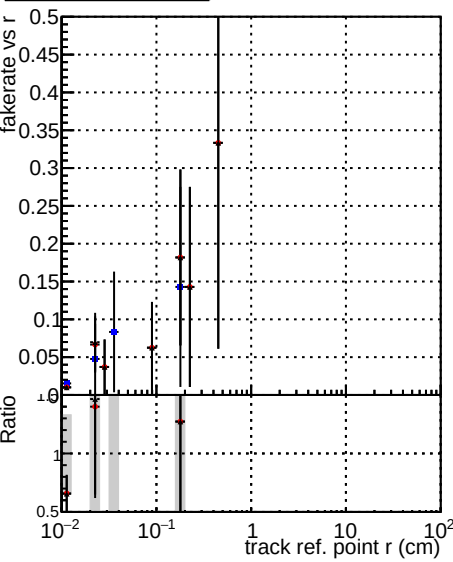
Fake rate vs verpos Global cmssw RECO Global mkFitOriginal RECO Global mkFitNewALL RECO Blue dots Red dots Black dots
