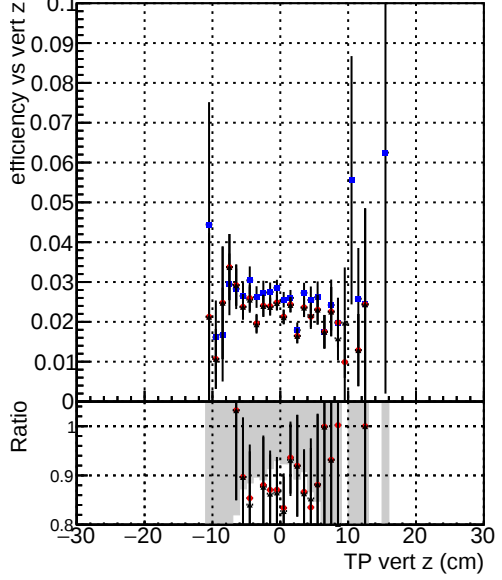
Efficiency vs. TP vert z (cm) —●— DQM_V0001_R000000001_Global_cmssw_RECO —●— DQM_V0001_R000000001_Global_mkFitOriginal_RECO —●— DQM_V0001_R000000001_Global_mkFitNewALL_RECO
