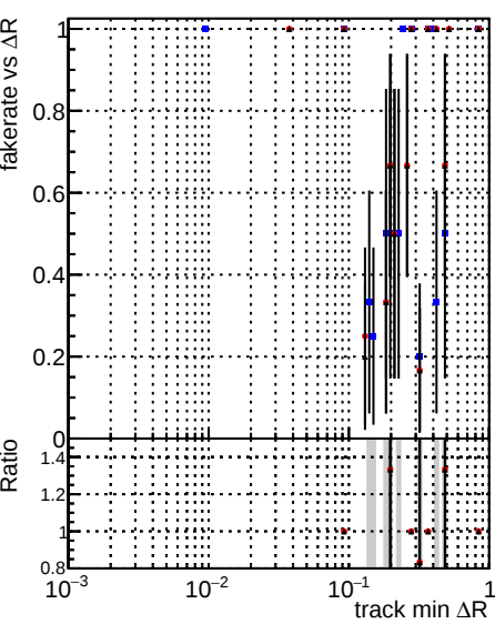
Fake rate vs \Delta R (track, jet) Global cmssw RECO DQM_V0001_R000000001 Global mkFitOriginal RECO DQM_V0001_R000000001 Global mkFitNewALL RECO
