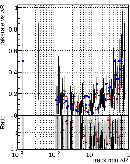
Fake rate vs \Delta R(\text{track, jet}) Duplicates Rate vs \Delta R(\text{track, jet}) Pileup rate vs \Delta R(\text{track, jet}) Legend: DQM_V0001_R000000001 Global cmssw RECO DQM_V0001_R000000001 Global mkFitOriginal RECO DQM_V0001_R000000001 Global mkFitNewALL RECO
