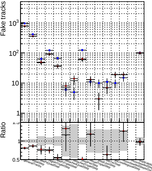
Number ● DQM_V0001_R0000000001_Global_mkFitOriginal_RECO ▲ DQM_V0001_R0000000001_Global_mkFitNewALL_RECO
