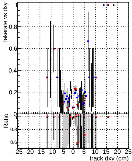
— DOM V0001 R0000000001 Global cmssw RECO — DOM V0001 R0000000001 Global mkFit Original RECO — DOM V0001 R0000000001 Global mkFit NewALL RECO
