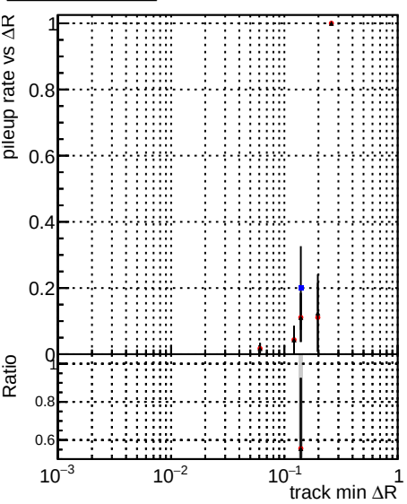
Fake rate vs \Delta R(\text{track, jet}) Duplicates Rate vs \Delta R(\text{track, jet}) Pileup rate vs \Delta R(\text{track, jet}) Legend for all plots: DQM_V0001_R000000001 Global cmssw RECO (Blue) DQM_V0001_R000000001 Global mkFitOriginal RECO (Red) DQM_V0001_R000000001 Global mkFitNewALL RECO (Black)
