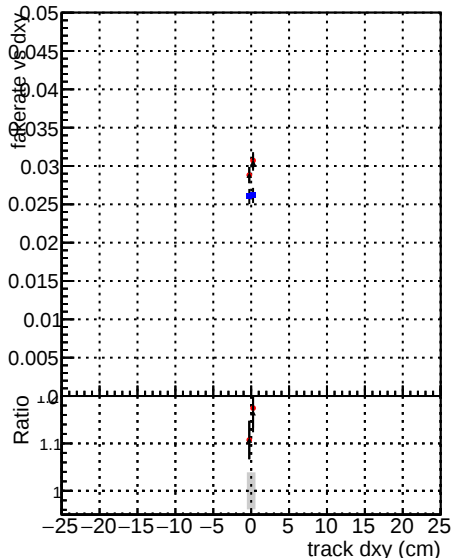
DOM_V0001 R0000000001 Global cms-sw RECO Fake rate vs d Blue Red Black Blue Red Duplicates Rate vs d Blue Red Black Blue Red Pileup rate vs d Blue Red Black Blue Red
