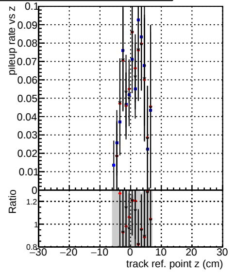
Legend: - Global cmssw RECO (blue circles) - Global mkFitOriginal RECO (red circles) - Global mkFitNewALL RECO (black circles)
