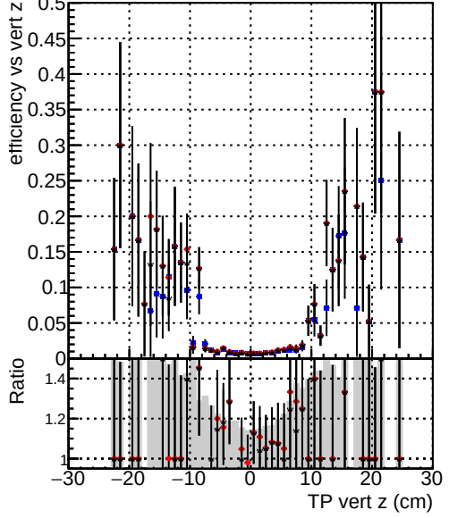
Efficiency vs vert z —●— DQM_V0001_R000000001_Global_cmssw_RECO —●— DQM_V0001_R000000001_Global_mkFitOriginal_RECO —●— DQM_V0001_R000000001_Global_mkFitNewALL_RECO
