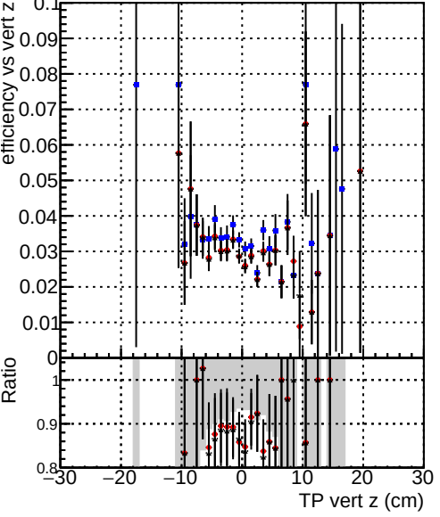
—●— DQM_V0001_R0000000001 Global_cmssw_RECO —●— DQM_V0001_R0000000001 Global_mkFitOriginal_RECO —●— DQM_V0001_R0000000001 Global_mkFitNewALL_RECO
