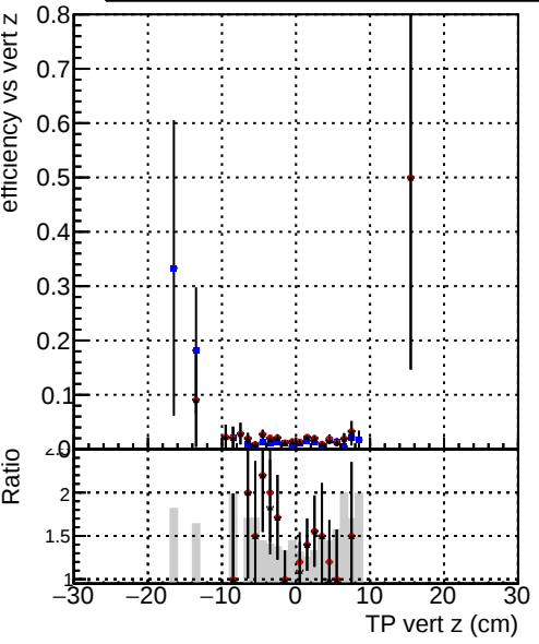
Efficiency vs vertpos Blue diamond DQM_V0001_R0000000001_Global_cmssw_RECO Red circle DQM_V0001_R0000000001_Global_mkFitOriginal_RECO Black triangle DQM_V0001_R0000000001_Global_mkFitNewALL_RECO
