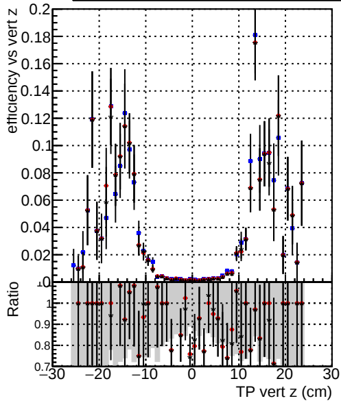
Efficiency vs vert z — DQM_V0001_R0000000001_Global_cmssw_RECO — DQM_V0001_R0000000001_Global_mkFitOriginal_RECO — DQM_V0001_R0000000001_Global_mkFitNewALL_RECO
