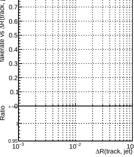
Fake rate vs \Delta R (track, jet)
