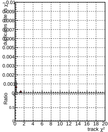
mkFitOriginal RECO a) mkFitNewALL RECO
