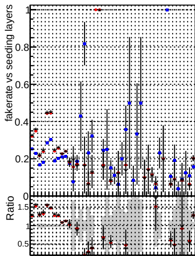
DOM V0001 R0000000001 Global cmissw RECO Fake rate vs. Blue stars Red stars Black stars Duplicates rate vs. Blue stars Red stars Black stars Pileup rate vs. Blue stars Red stars Black stars
