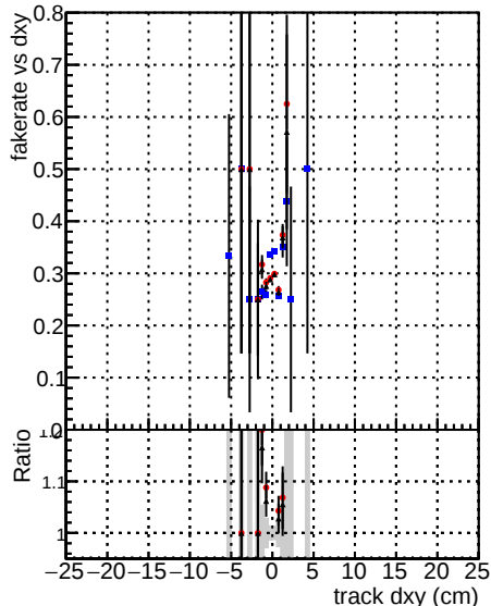
Fake rate vs d Legend DOM V0001 R0000000001 Global cmssw RECO Blue square DOM V0001 R0000000001 Global mkFitOriginal RECO Red circle DOM V0001 R0000000001 Global mkFitNewALL RECO Black triangle DOM V0001 R0000000001 Global mkFitNewALL RECO
