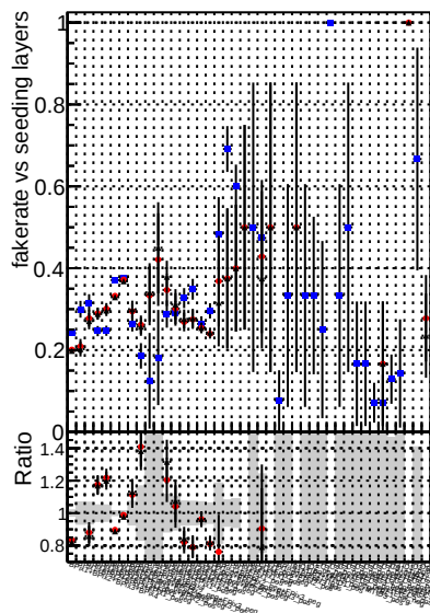
Fake rate vs. Legend DOM V0001 R0000000001 Global cms-sw RECO Global mkfOriginal RECO Global mkfNewALL RECO Blue circle DOM V0001 R0000000001 Global cms-sw RECO Global mkfOriginal RECO Global mkfNewALL RECO Red circle DOM V0001 R0000000001 Global cms-sw RECO Global mkfOriginal RECO Global mkfNewALL RECO Black circle DOM V0001 R0000000001 Global cms-sw RECO Global mkfOriginal RECO Global mkfNewALL RECO
