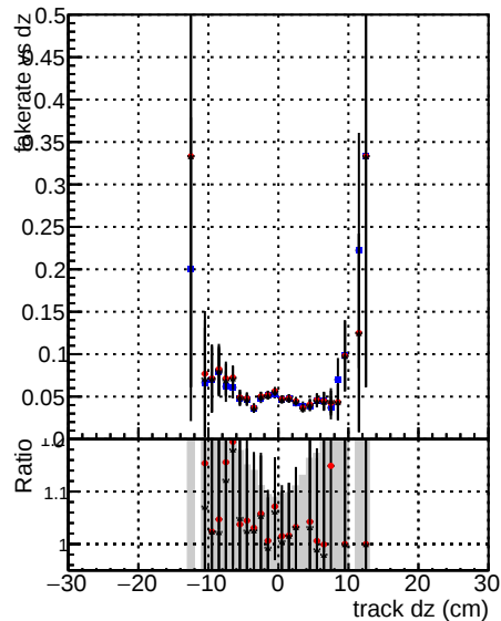
Fake rate vs dz —●— DOM mkFit newBASE3 —●— DOM mkFit newWANDPL
