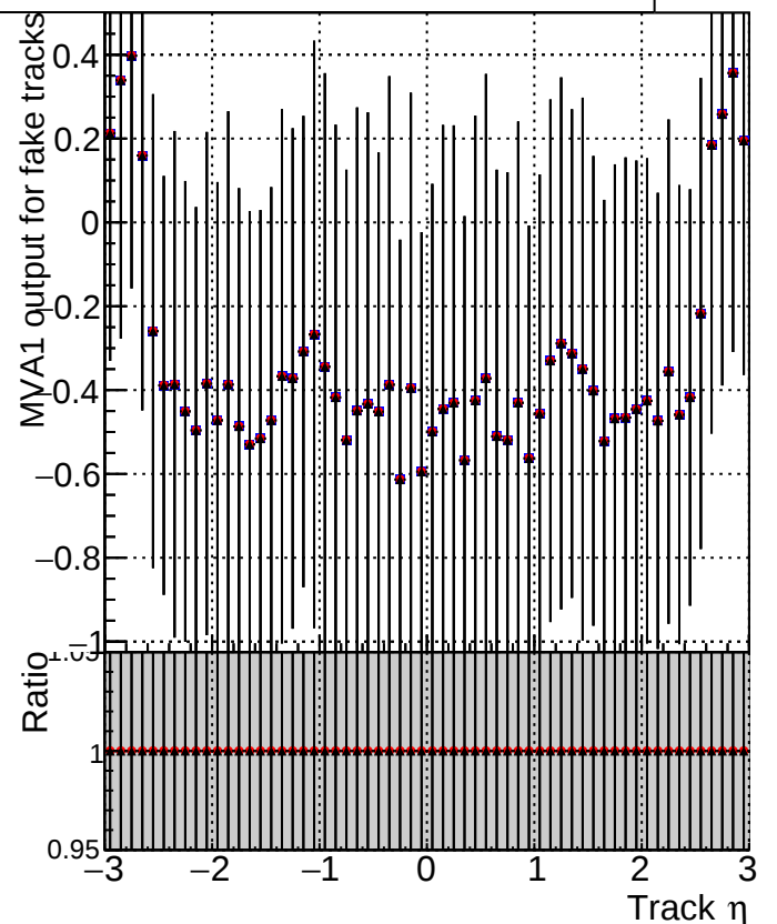
MVA1 of associated tracks (recoToSim) vs. track \eta Legend: DQM_mkFit_newBASE3 (Blue square) DQM_mkFit_new (Red circle) DQM_mkFit_newANDPL (Black triangle)
