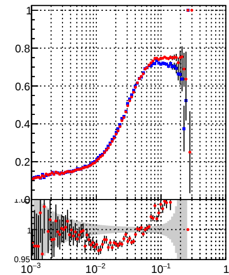
—•— DQM_TT_mkFit_BDT_ —•— DQM_TT_mkFit_
