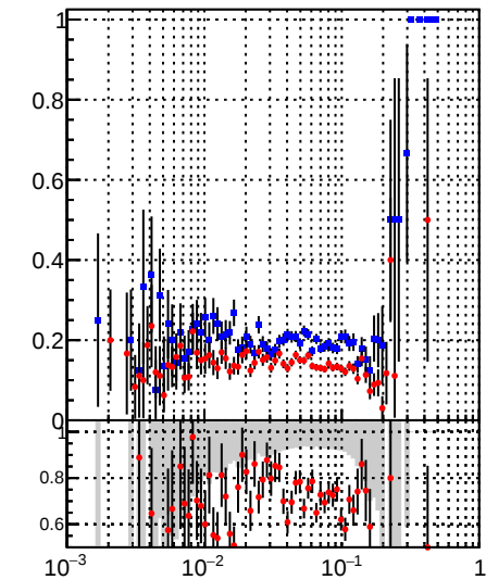
Fake rate vs \sqrt{s} Legend: DQM_TT_mkFit_BDT_ (blue) DQM_TT_mkFit_ (red)
