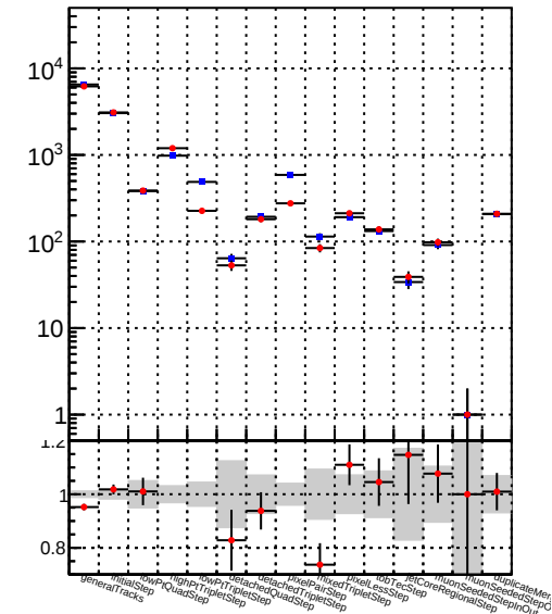
Number —●— DQM_TT__mkFit_
