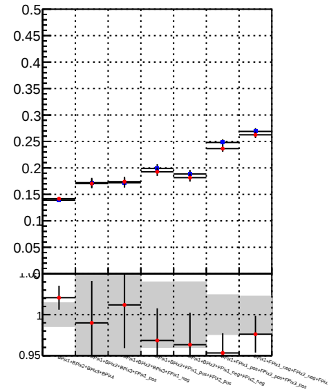
Fake rate vs. DQM_TT_mkFit_BDT_ DQM_TT_mkFit_
