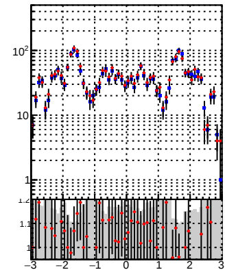
N of reco track vs \eta DQM_TT_mkFit_BDT_ DQM_TT_mkFit_
