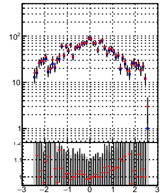
N of reco track vs \eta DQM TT mkFit BDT
