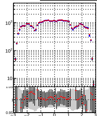
—•— DQM_TT_mkFit_BDT_ —•— DQM_TT_mkFit_
