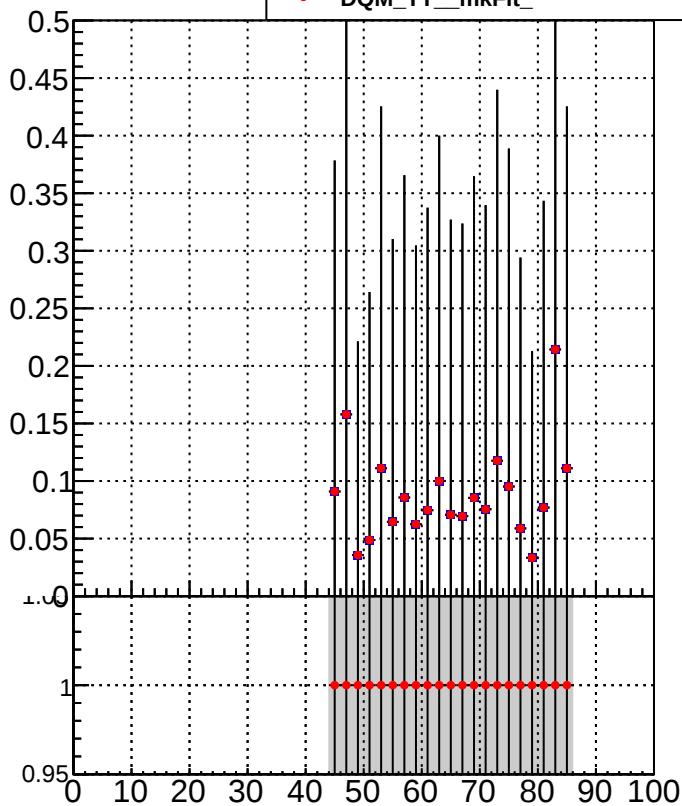
■ DQM_TT_mkFit_BDT_ ● DQM_TT_mkFit_
