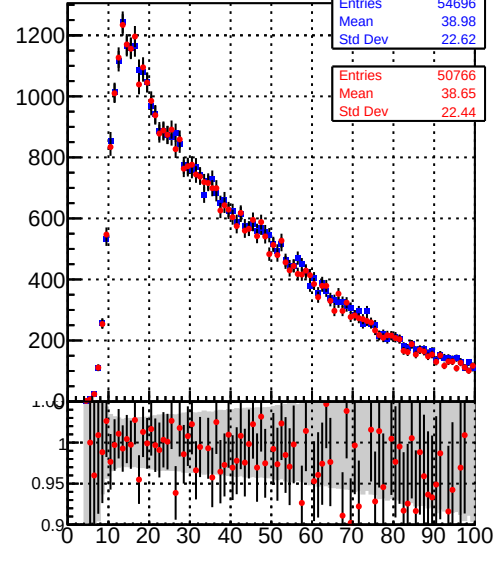
Uncertainty z Coordinate (tagged Vtx) DQM_TT_mkFit_BDT_ DQM_TT_mkFit_
