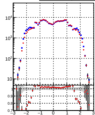
◆ DQM_TT_mkFit_BDT_ × DQM_TT_mkFit_
