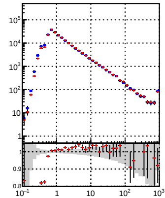
◆ DQM_TT_mkFit_BDT_ × DQM_TT_mkFit_
