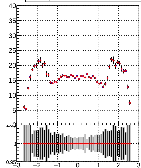
mean hit — DQM_TT_mkFit_BDT_ — DQM_TT_mkFit_
