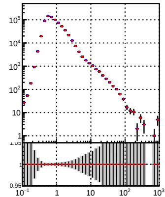
—●— DQM_TT_mkFit_BDT_ —●— DQM_TT_mkFit
