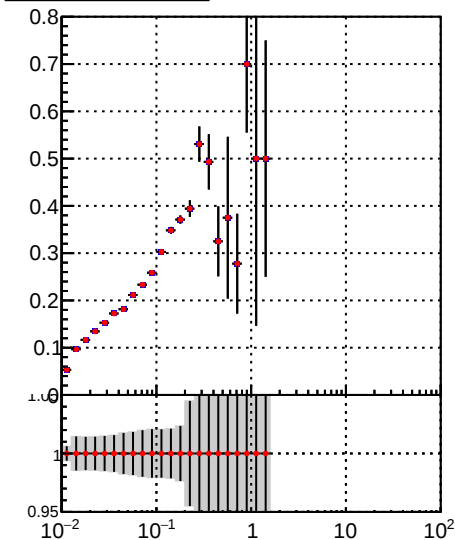
█ DQM_TT_mkFit_BDT_ █ DQM_TT_mkFit_ Fake rate vs \nu
