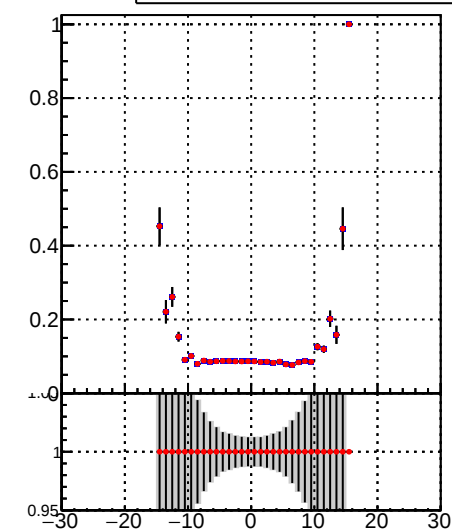
█ DQM_TT_mkFit_BDT_ █ DQM_TT_mkFit_ Fake rate vs \nu
