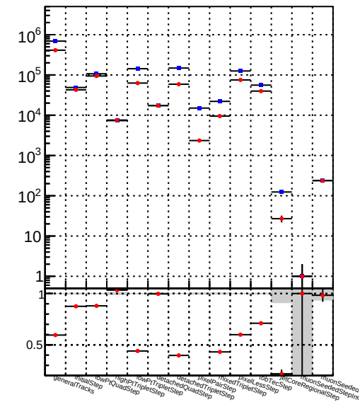
Number —●— DQM_TT_mkFit_
