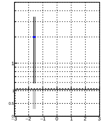
N of associated (recoToSim) duplicate tracks vs \eta —•— DQM_TT_mkFit_BDT_ —+— DQM_TT_mkFit_
