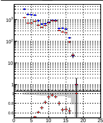
◆ DQM_TT_mkFit_BDT_ + DQM_TT_mkFit_ 1 layer
