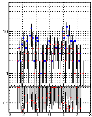
N of reco track vs \eta —•— DQM_TT_mkFit_BDT_ - - - DQM_TT_mkFit
