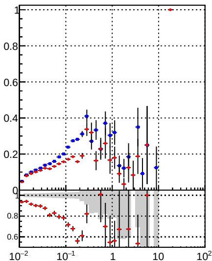
—●— DQM_TT_mkFit_BDT_ —●— DQM_TT_mkFit_
