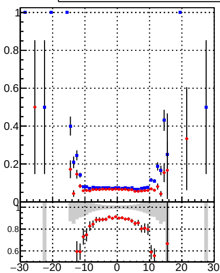
—●— DQM_TT_mkFit_BDT_ —●— DQM_TT_mkFit_
