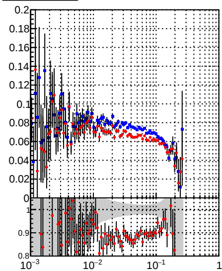
Fake rate vs DQM_TT_mkFit_BDT_ DQM_TT_mkFit_
