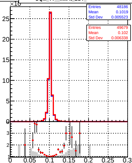
Recons DQM_TT_mkFit_ DQM_TT_mkFit_BDT_
