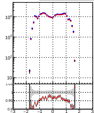
—•— DQM_TT_mkFit —+— DQM_TT_mkFit_BDT
