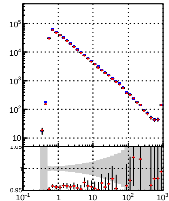
—•— DQM_TT_mkFit —+— DQM_TT_mkFit_BDT
